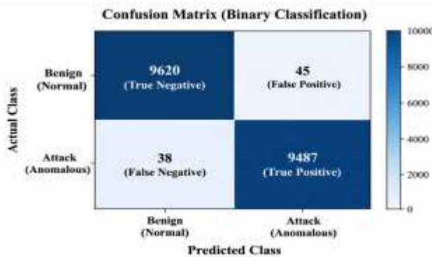
Figure 3: Binary Classification Confusion Matrix
