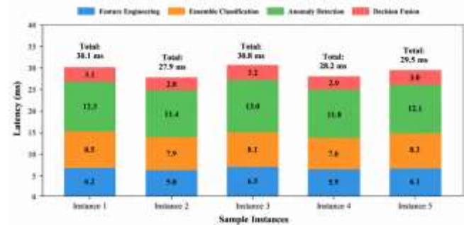
Figure 6: Processing Latency by Pipeline Stage
