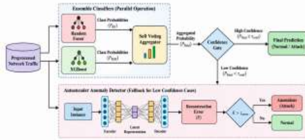
Figure 2: Hybrid Detection Architecture
