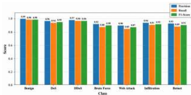
Figure 4: Per-Class Detection Performance
