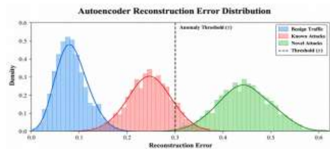
Figure 5: Autoencoder Reconstruction Error Distribution
