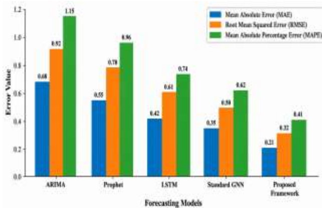
Figure 3: Comparative Performance of Forecasting Models
