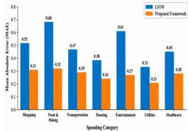
Figure 5: Category-Level Prediction Performance
