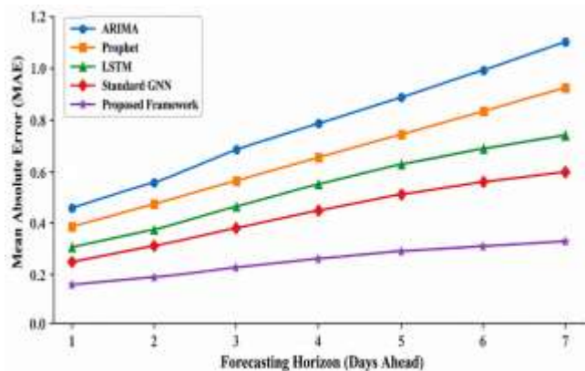
Figure 4: Prediction Accuracy Across Forecasting Horizons
