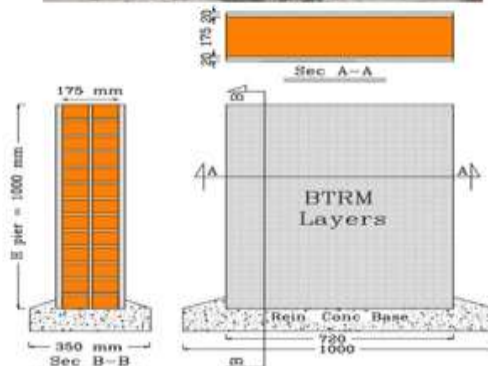
Figure 2: Basalt textile mesh and BTRM strengthening configuration.
