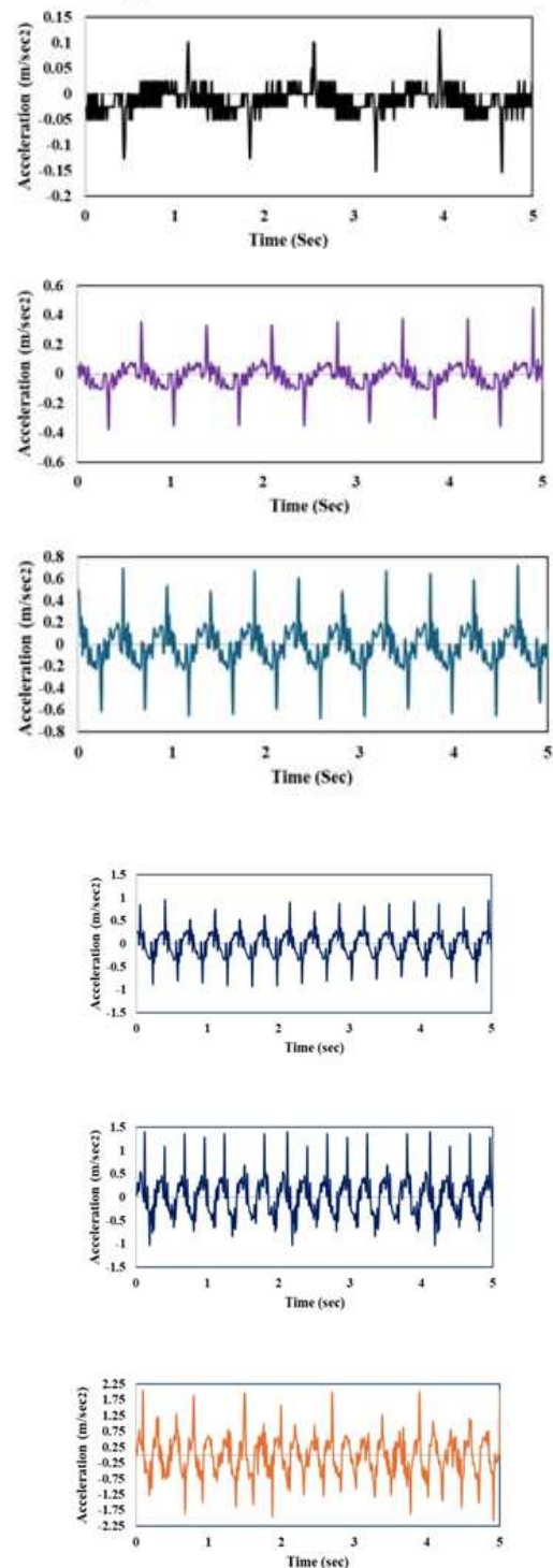
Figure 4: Input acceleration time histories of the shaking table at excitation frequencies of (a) 0.70 Hz, (b) 1.40 Hz, (c) 2.10 Hz, (d) 2.80 Hz, (e) 3.50 Hz, and (f) 4.20 Hz
