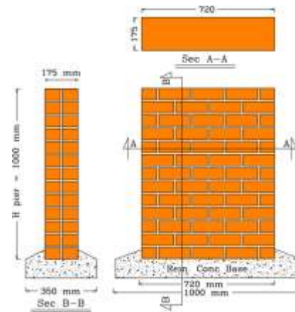
Figure 1: Geometry and dimensions of the masonry pier specimens.
