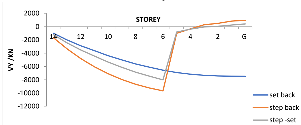
Figure 5.9: “Variation of Storey Shear for Three Buildings under Load combination (0.9 DL + 1.5 ELY)”
