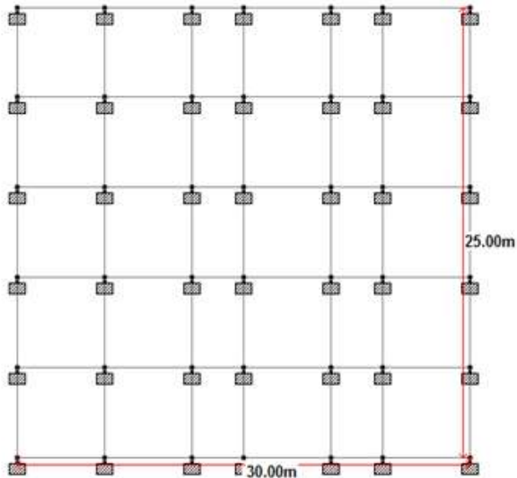
Figure 4.1: “Plan of Configuration of Building”
