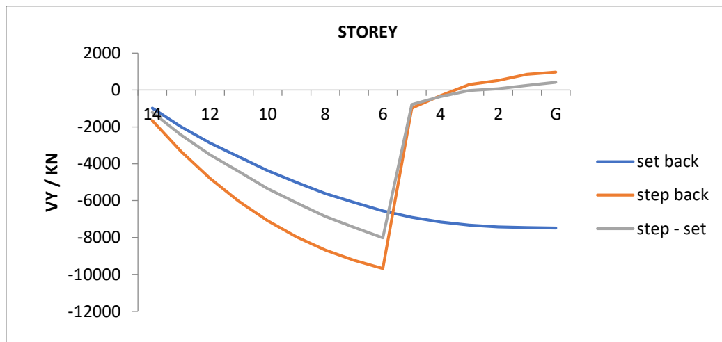
Figure 5.8: “Variation of Storey Shear under Load of combination 1.5 (DL + ELY)”
