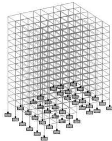
Figure 4.4: “Step-set Back Building Isometric view”
