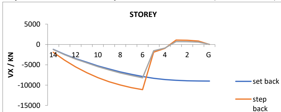
Figure 5.6: “Variation of Storey Shear under Load of combination (0.9 DL + 1.5 ELX)”
