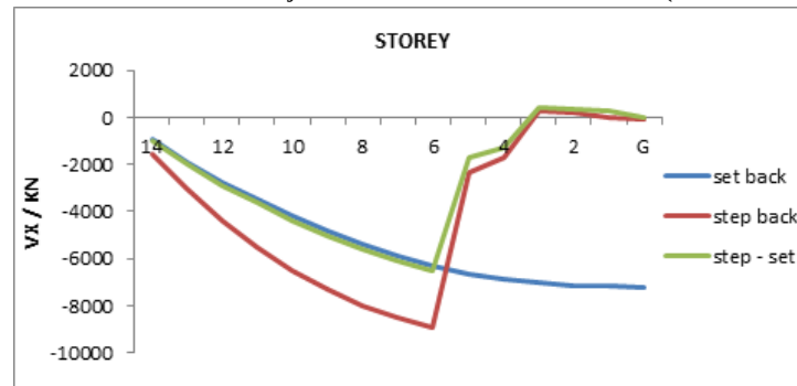
Figure 5.7: “Variation of Storey Shear under Combination Load 1.2 (DL+LL+ELX)”
