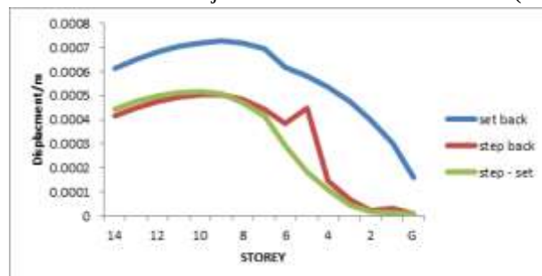
Figure 5.1: "Storey Drift under Load of combination 1.2 (dl + ll + elx )"
