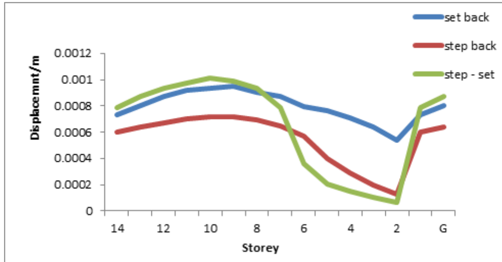
Figure 5.3: “Storey Drift in Y Direction under Load of combination 1.2 (dl + ll +ely)”
