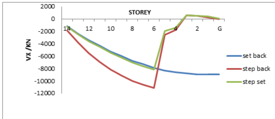
Figure 5.5: “Variation of Storey Shear under Load of combination 1.5 (DL+ ELX)”
