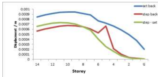
Figure 5.2: “Variation of Storey Drift for Load of combination (0.9dl+1.5 elx)”
