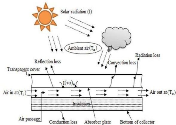
Fig. 1. Schematic of a simple solar air heater
