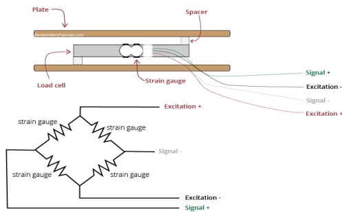
Figure6: load cell sensor
