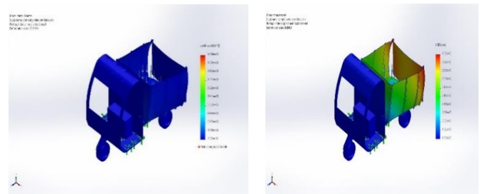
Figure10: simulation of dumper bucket
