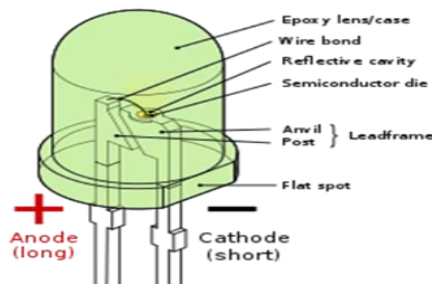
Figure9: LED
