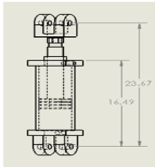
Figure3: draft sketch of cylinder
