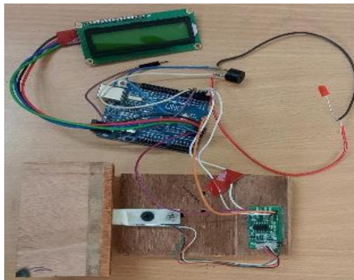
Figure 11: circuit connection
