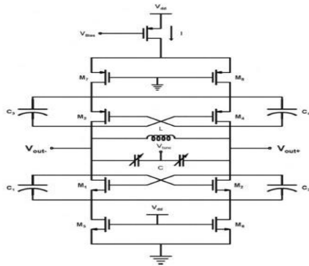
Fig.4. Cross coupled LC tank VCO with double Pseudo resistance.
