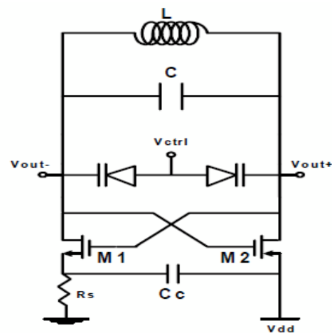
Fig.2. Cross coupled differential topology
