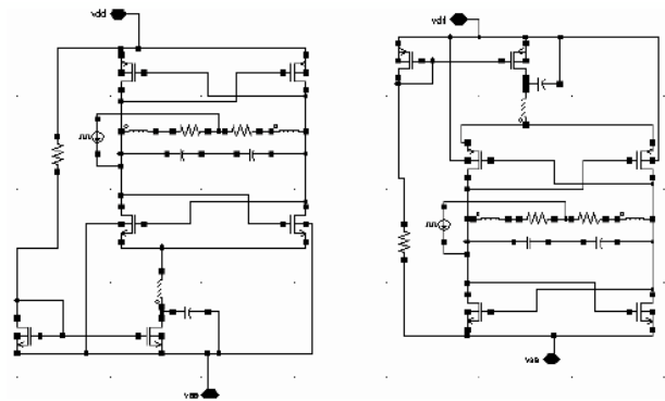
Fig.3. Complimentary cross coupled LC tank VCO.
