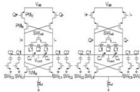
Fig.5. Quadrature VCO using Reconfigurable LC tank
