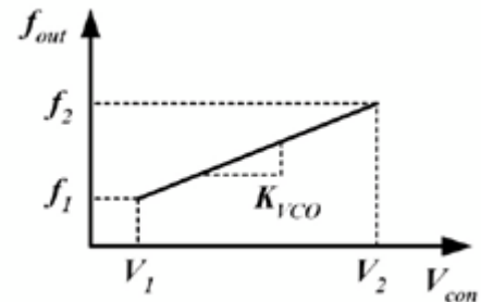
Fig.6. Definition of K_{VCO}
