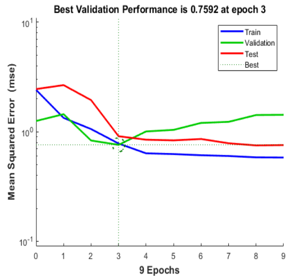
Fig.6 Variation of MSE with respect to epochs.
