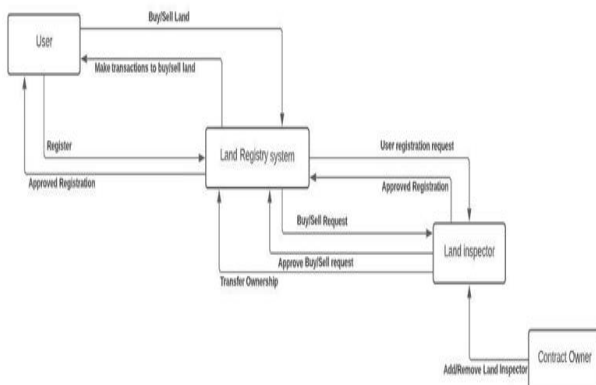
Fig 1. Context Level Diagram.
