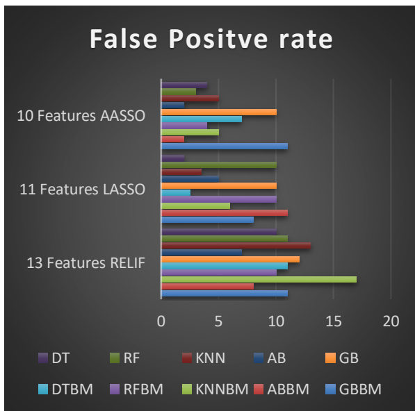
Fig 8. Comparison of False positive rate.
