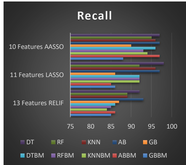
Fig 6. Comparison of Recall.
