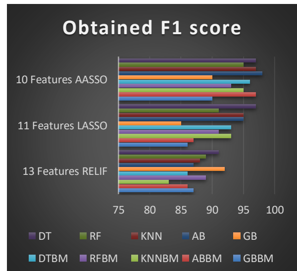
Fig 7. Comparison of F1 Score.
