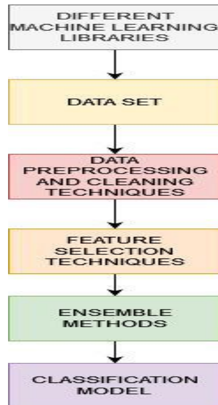
Fig 4. Implementation Techniques
