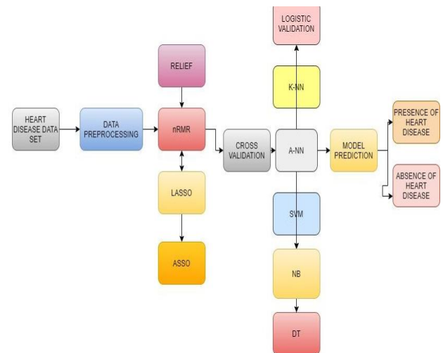
Fig 2. Proposed model.
