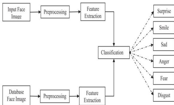
Fig 1. The architecture of facial expression recognition system.
