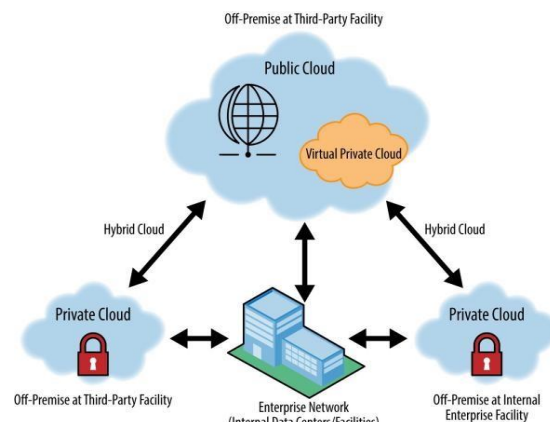
Fig 3. Model.
