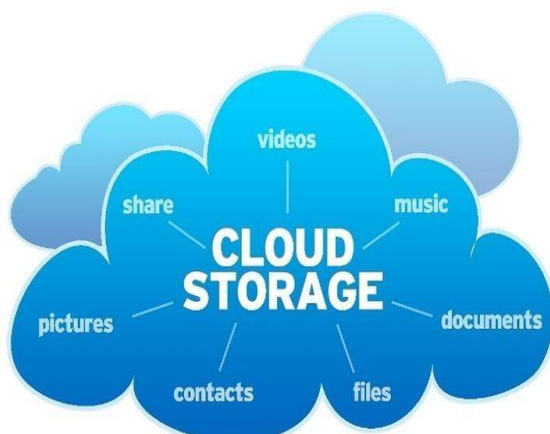
Fig 1. Cloud Storage.
