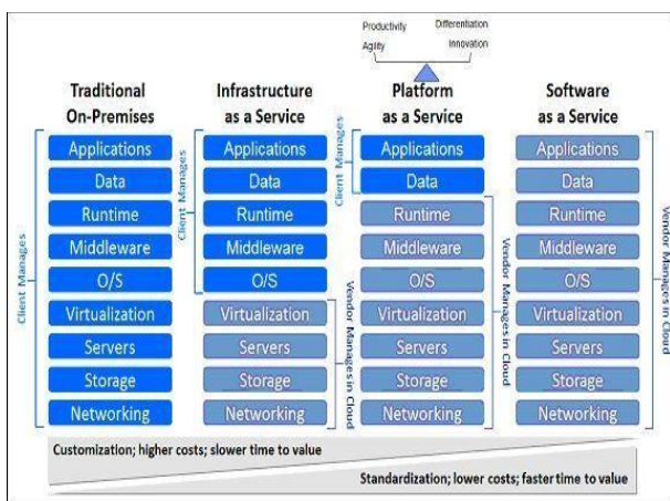
Fig 2. Infrastructure.
