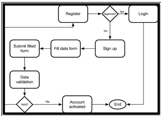
Figure 1 Workflow Diagram Of Registration Process .
