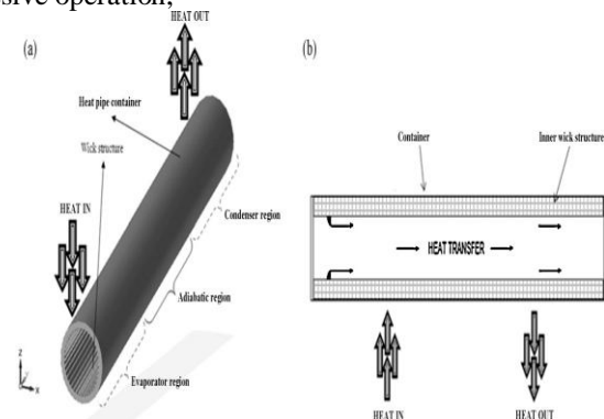
Fig. 1. Basic working principle associated with a heat pipe (a) isometric view and (b) sectional view.
