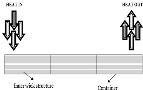
Fig. 2 Schematic of a tubular heat pipe.
