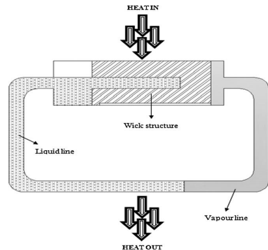
Fig. 4 Schematic of a loop heat pipe arrangement.
