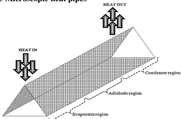
Fig. 5. Schematic of a micro heat pipe.
