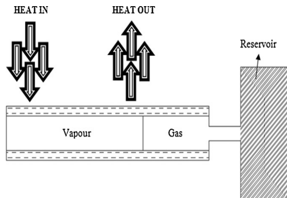
Fig. 3. Schematic of a cold-reservoir variable conductance heat pipe.
