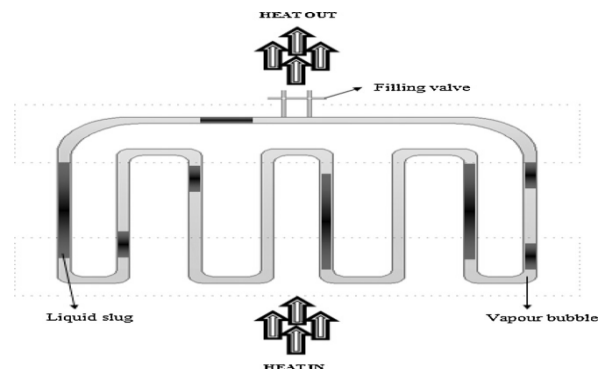
Fig. 3. Schematic of a Variable-conductivity heat pipes
