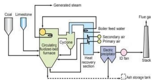
Fig 3. Process Flow of Circulating Fluidized- Bed Boiler.
