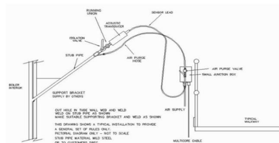
Fig 1. Fitting and locating the sensor.
