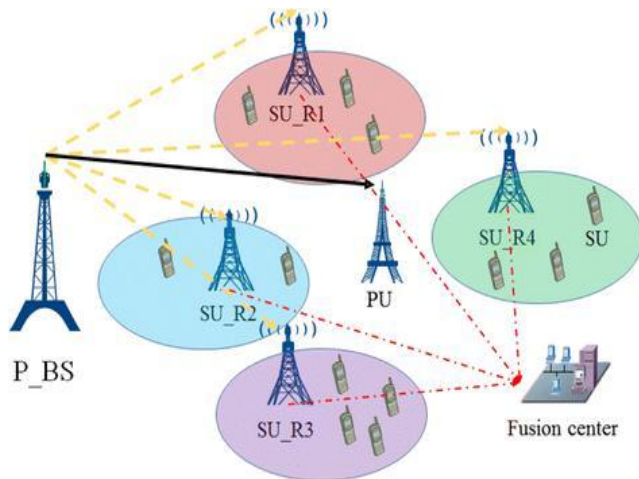
Figure 2 Centralized Cooperative spectrum sensing
