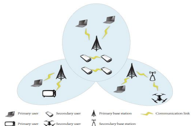
Fig 1 cognitive network
