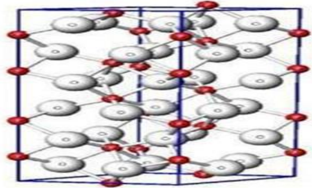
Fig. 2 Crystal structure of Hematite.
