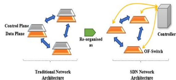
Figure 9. Traditional network architecture versus SDN, network architecture.
