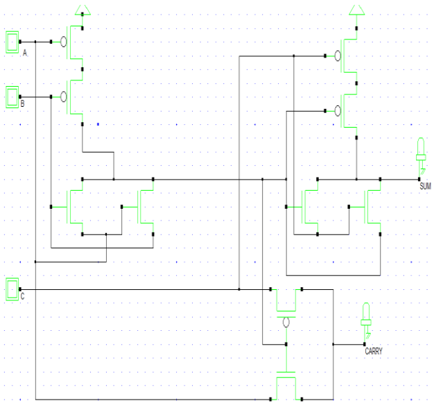
Figure 2 Architecture Design of 1-bit Full Adder using ten transistors.
