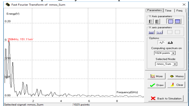
Figure 11 Shows the Fast Fourier Transform of nmos_sum of 1-Bit Proposed FA.
