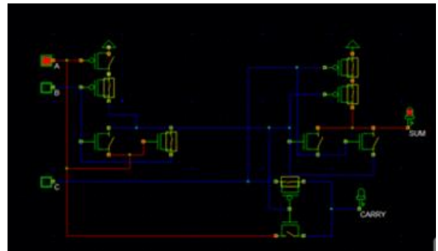
Figure 3 DSCH Full Adder Design.
