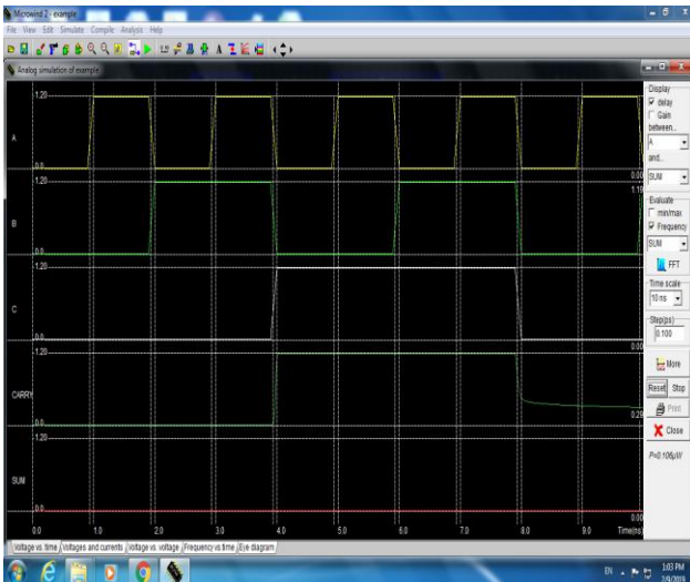
Figure 6 Results Waveform Voltage Vs Time of 1-Bit Proposed FA (90 nm).
