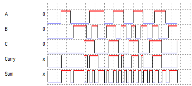
Figure 4 Timing Diagram of DSCH Full Adder Design.
