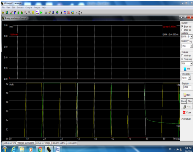
Figure 7 Results Waveform Voltage Vs Current of 1-Bit Proposed FA (90 nm).
