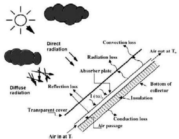
Fig. 1.1 Solar air heater constructional details.
