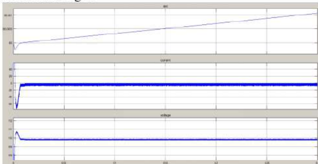
Fig. 17. Battery(SOC,Current,Voltage)
