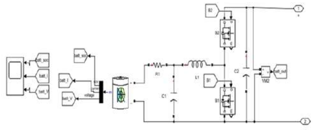
Fig.5. Battery Subsystem.
