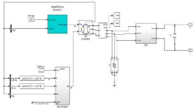
Fig.4 .Diesel Generator system.
