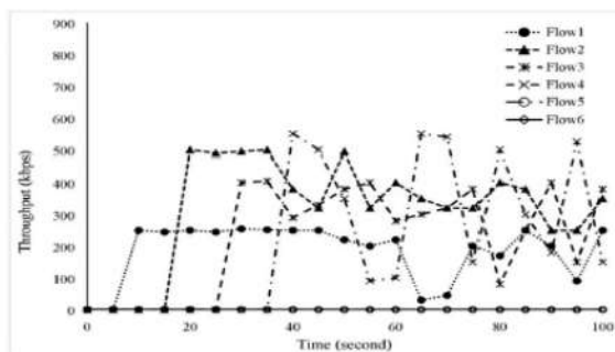
Fig. 4.3. Throughput of flows using IAB [7] for admission control.
