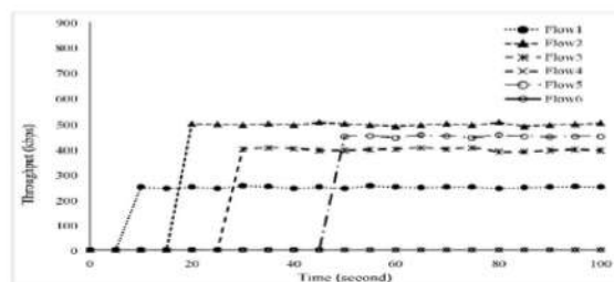
Fig. 4.5. Throughput of flows using proposed AABWM for admission control.
