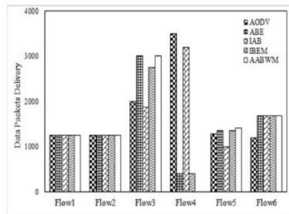
Fig. 4.12. Data packet delivery
