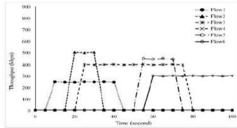
Fig. 4.10. Throughput of flows using proposed AABWM approach for admission control.
