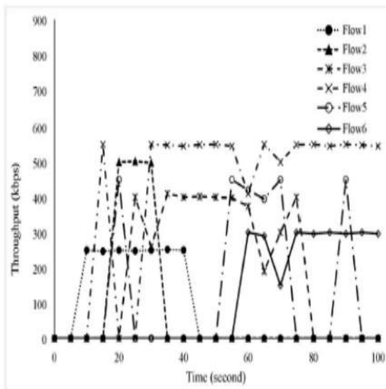
Fig.4.6. Throughput of flows using AODV [22] without any admission control.
