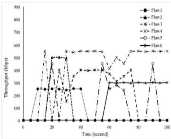
Figure 4.8. Throughput of flows using IAB [7] for admission control.
