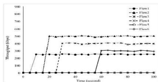
Fig.4.4. Throughput of flows using IBEM [18] for admission control.
