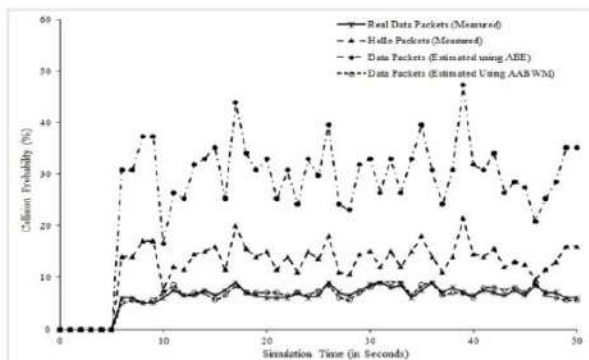
Fig.2. Estimated results of collision probabilities of packets.
