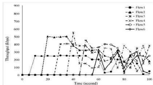
Fig.4.1. Throughput of flow using AODV [22] without any admission control
