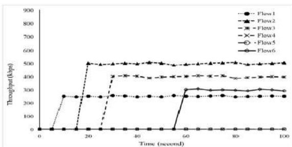
Fig.4.2. Throughput of flows using ABE [4] for admission control.
