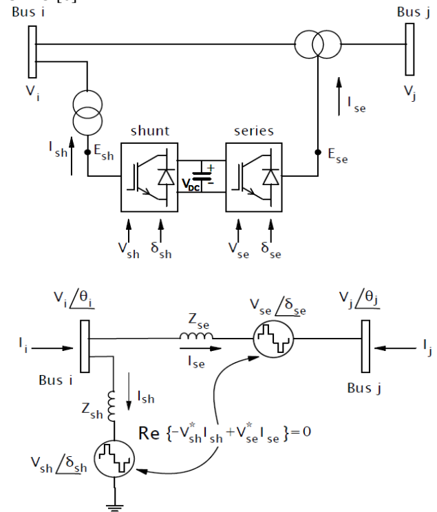
Figure 4 UPFC Equivalent Circuit. (a) UPFC schematic diagram; (b) UPC equivalent circuit
