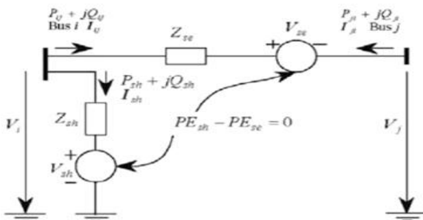
Figure 3 Equivalent circuit of a UPFC [14]
