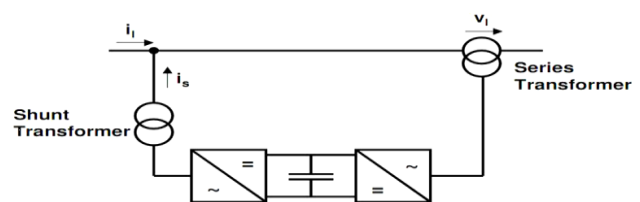
Figure 1. Principle configuration of an UPFC [19]
