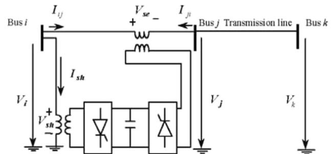
Figure 2 Operating principle of a UPFC [20]
