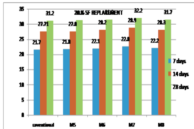
Fig.3&4-compressive strength on concrete with 10% and 20% replacement
