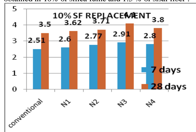
Fig. 5 Split tensile strength on concrete with 10% replacement
