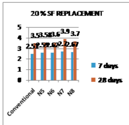
Fig. 6 Split tensile strength on concrete with 20% replacement.
