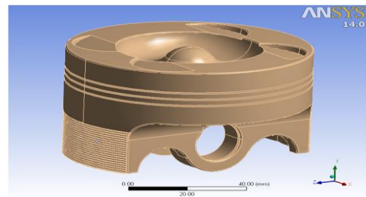
Fig.4. Piston after optimization in ANSYS.
