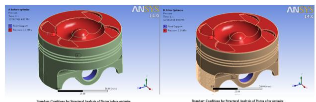
Fig.6. Structural Boundary Condition before and after optimize in ANSYS.
