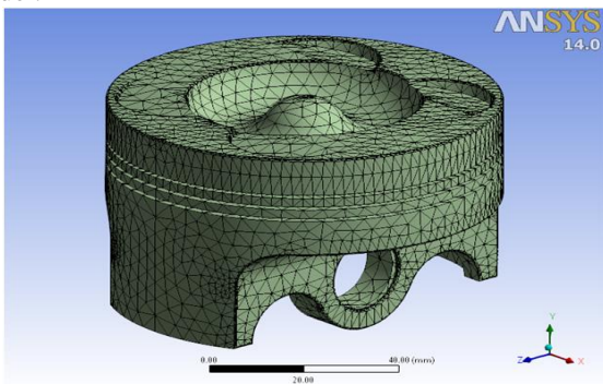
Fig.3. Shows meshed model of the piston.
