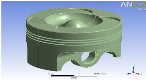
Fig.2. Piston before optimize in ANSYS.
