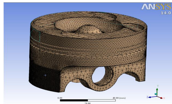
Fig.5. shows meshed model of the piston after optimization.
