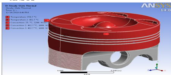
Fig.7. Thermal Boundary Condition after optimizing in ANSYS.
