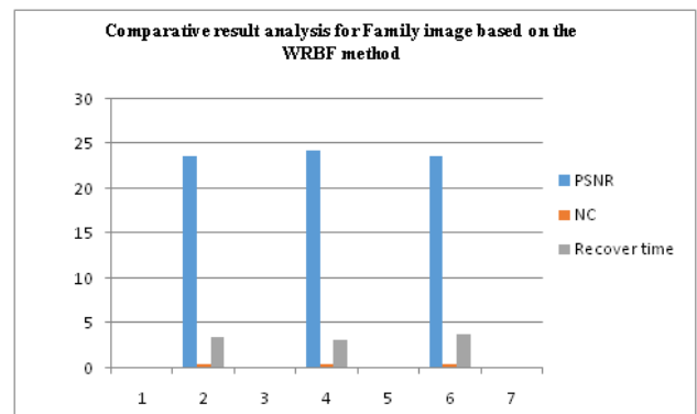
Fig. 6: Shows that a comparative result analysis for Family image based on the WRBF method. We find the value of PSNR, NC and Recover time. These all value find with the some feture such as Cropping, Shear and Noise.
