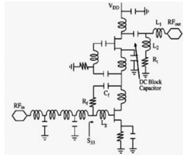
Fig.2. Simplified schematic of the wideband LNA [4].
