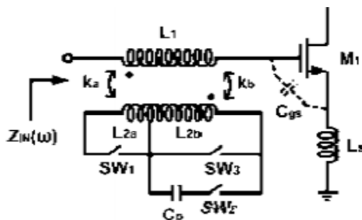
Fig. 4. Multimode LNA with a reconfigurable multi-tap transformer as the gate inductor [6].
