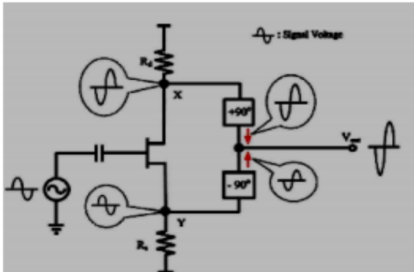
Fig.3. Illustration of forward combining technique [5].
