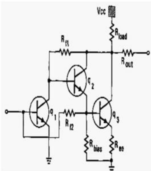
Fig.1. Schematic of the direct-coupled HBT amplifier [3].
