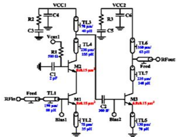
Fig.5. Schematic of the two-stage low-noise amplifier [7].
