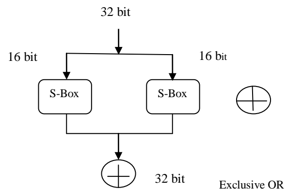
Fig.3 S-boxes break in Two Parts.
