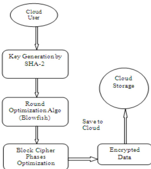
Fig.2 Working Architecture of algorithms for encryption.
