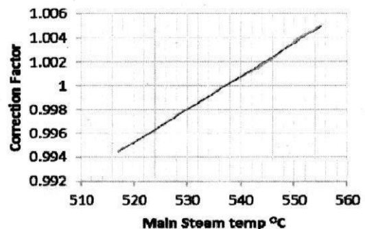
Fig. 2 Correction Curve for MS Temperature.
