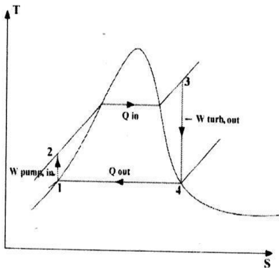
Fig 1 Rankine Cycle.
