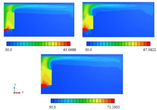
Fig.4 Temperature distribution of three Optimum solutions.
