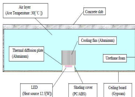
Fig.1 Heat sink setup.
