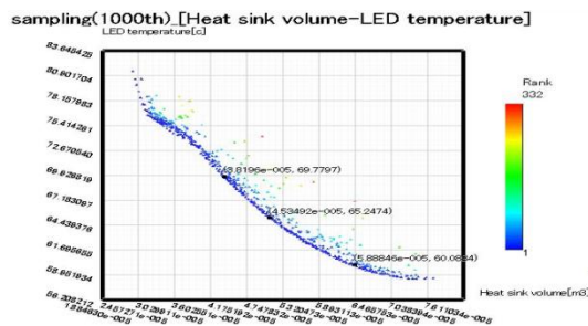
Fig.3 the final solutions of MOGA generation.
