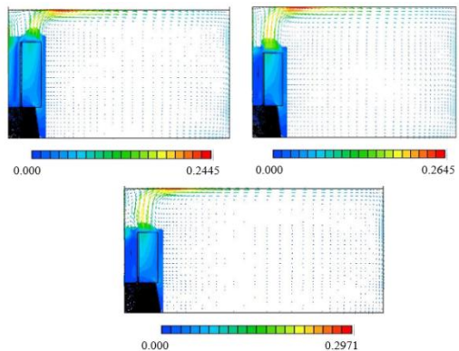
Fig.5 Flow distribution of three optimum solutions.
