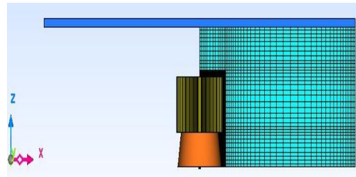
Fig.2 Meshed LED Heat sink model.
