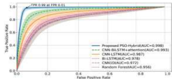
Figure 4: Comparative ROC Curves for Intrusion Detection Models.
